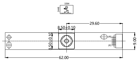
PH1.0,Side entry type, 5 PINS
